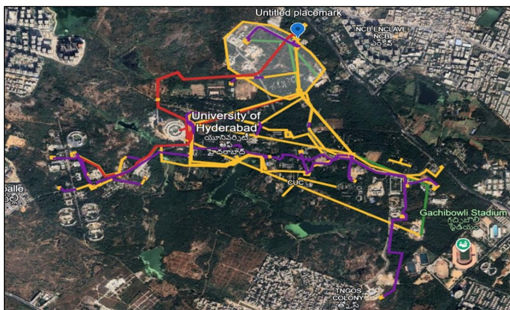
Figure 3 Existing Grid Network
